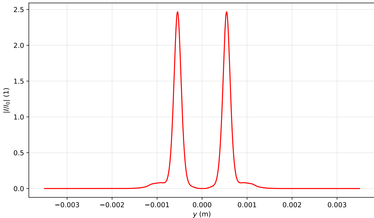
Intensity profile I(x=0, y, z=0.637)/I_0 , \text{Pin}=9.0\text{Pcr} , artificial time
